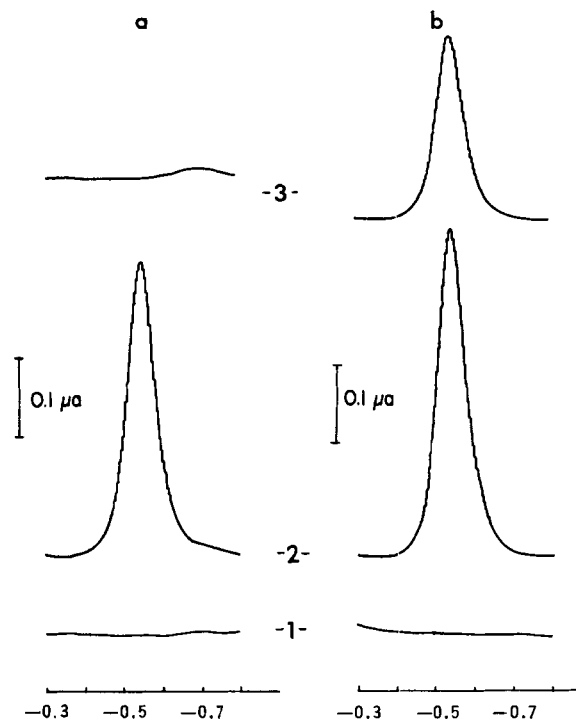
Figure 2—Polarograms of I and carbamate anion II in acetate and ammonia buffers. Key: a, acetate-ethanol buffer; b, ammonia-ethanol buffer; 1, blank; 2, I in corresponding buffer (10 mcg./ml.); and 3, carbamate anion II in corresponding buffer (10 mcg./ml.).
